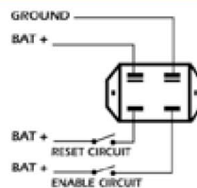
4 TERMINAL
