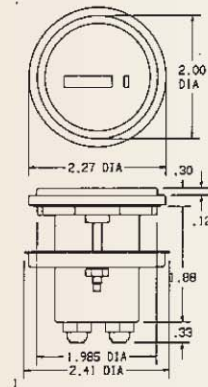
Flush Mount (Cup) 2.27": Panel cutout 2.00 diameter opening. *
