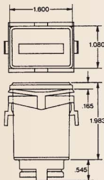
Rectangular Retainer: Panel cutout 1.45 x .95 rectangular opening
