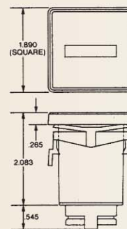
Square Retainer: Panel cutout 1.45 x .95 rectangular opening
